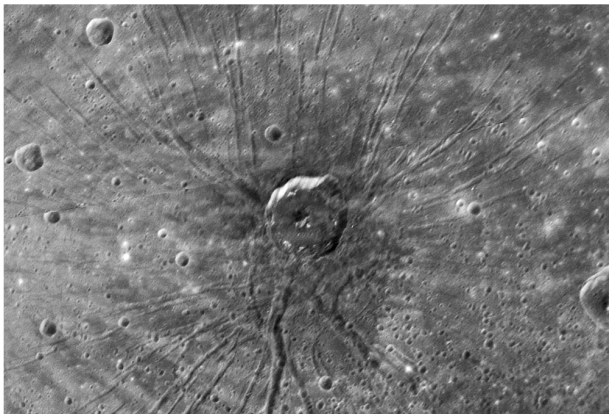
Система борозд (гребен) "Паук" (The Spider). MESSENGER, NASA/Johns Hopkins University Applied Physics Laboratory/Carnegie Institution of Washington http://www.shvedun.ru/images/stat/merc/mercury-3.jpg
